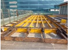
2. Pool after PCC
