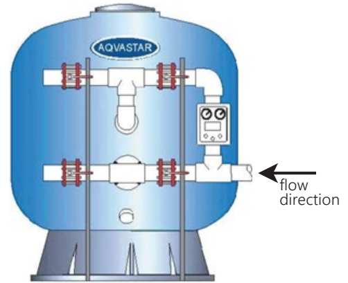
4 VALVE BATTERY
