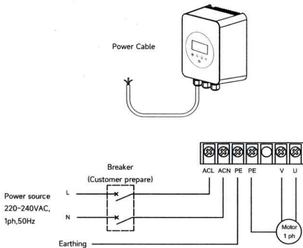
Fig. 4 1-ph pump connection diagram
