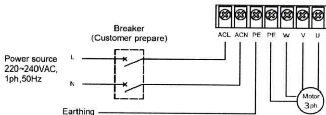
Fig. 5 3-ph pump connection diagram
